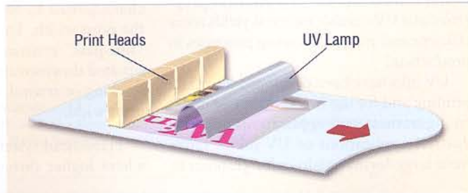
Figure 2: Fixed-head High-Speed Ink Jet
