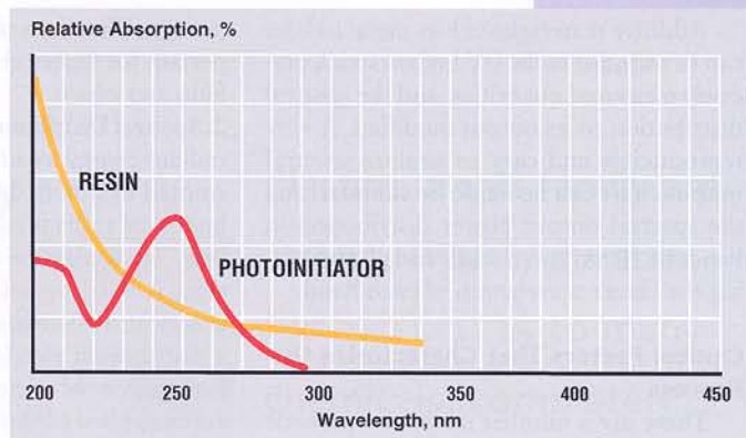
Figure 4: A "Clear" Film May Use Short-Wavelength Photoinitiators and Exposure
