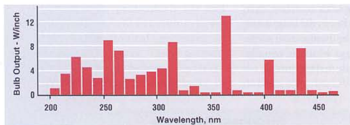
Figure 7: Spectral Distribution of Emission of a Medium-Pressure Mercury Bulb
