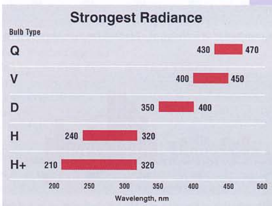
Figure 6: Additives in Mercury Bulbs Are Used to Control Their Spectral Output
