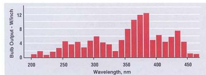
Figure 8: Spectral Distribution of Emission of a Mercury Bulb with an Iron Halide Additive
