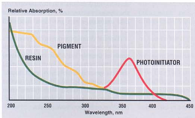
Figure 5: Inks Benefit from Long-Wavelength Photoinitiators and Exposure
